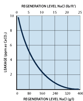
Fig. 5 HARDNESS LEAKAGE
