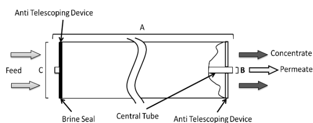
Figure 2: Element Dimensions Diagram – Male
