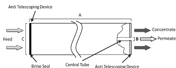
Figure 1: Element Dimensions Diagram – Female
