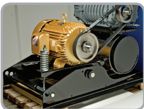
Automatic belt tensioning system is counter-balanced to extend V-belt life
